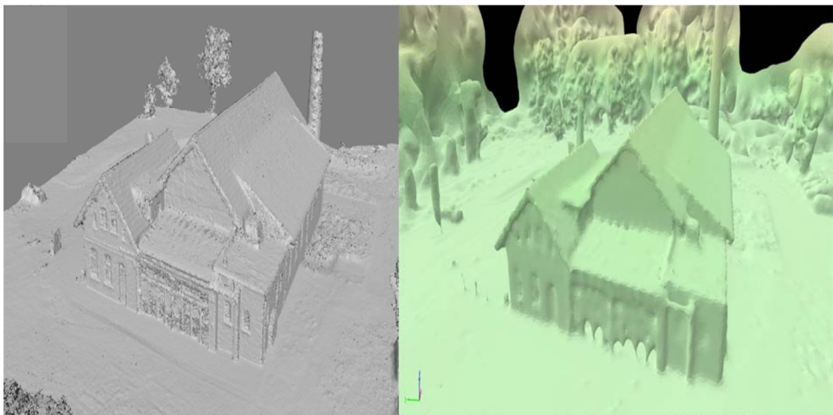
Fig. 3. Image (Dense Cloud) generated by the tested software: on the left – Agisoft Photo Scan Professional Edition, on the right – Pix4D Pro mapper
