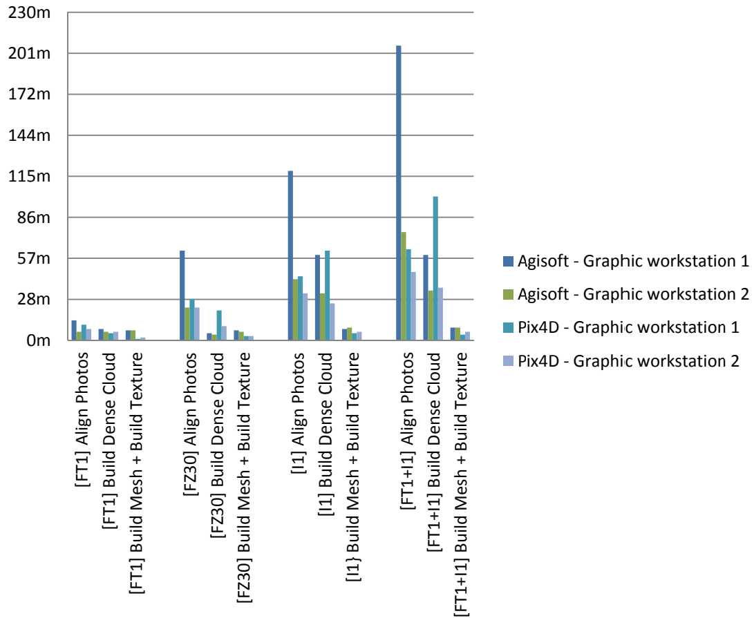
Chart 1. Times of processing of different blocks of images, broken down into stages, software and graphic workstations
